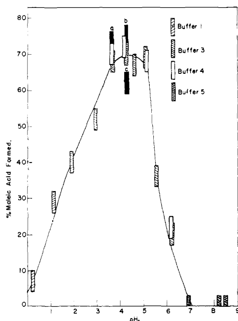
Fig. 1.—Relation of percentage maleic acid formed to pH in the macro scale reduction of rac -dibromosuccinic acid. Data are at 25^\circ except that a represents a run in buffer 4 at 2.0^\circ ; b , buffer 3, 2.0^\circ ; c , buffer 3 made 2.0 M with KCl , 25.0^\circ . Points are drawn to show a possible \pm 3\% deviation in determination of maleic acid formed, and \pm 0.05 unit deviation in pH .
