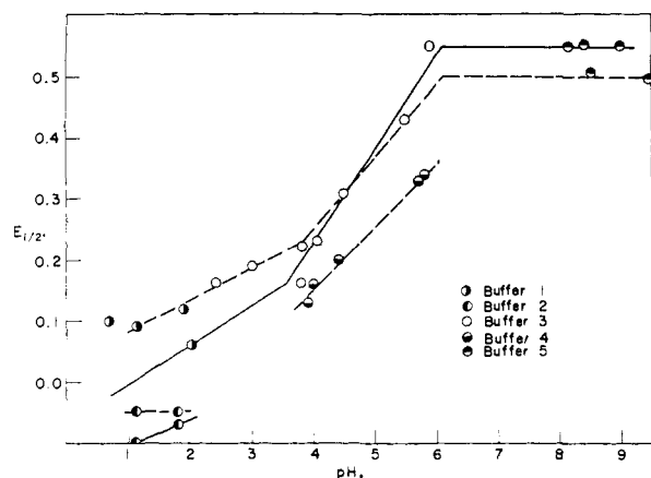
Fig. 2.—Variation of E_{1/2} with pH for rac - and meso -dibromosuccinic acids. The solid line is based on experimental data taken from reference 4b on the meso acid; plotted points represent experimental values obtained in the present study. The broken line represents data found for the racemic acid.
