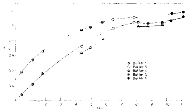
Fig. 4.—Variation of E_{1/2} with pH for diethyl maleate and diethyl fumarate. The solid line represents data for diethyl fumarate, the broken line for diethyl maleate.
