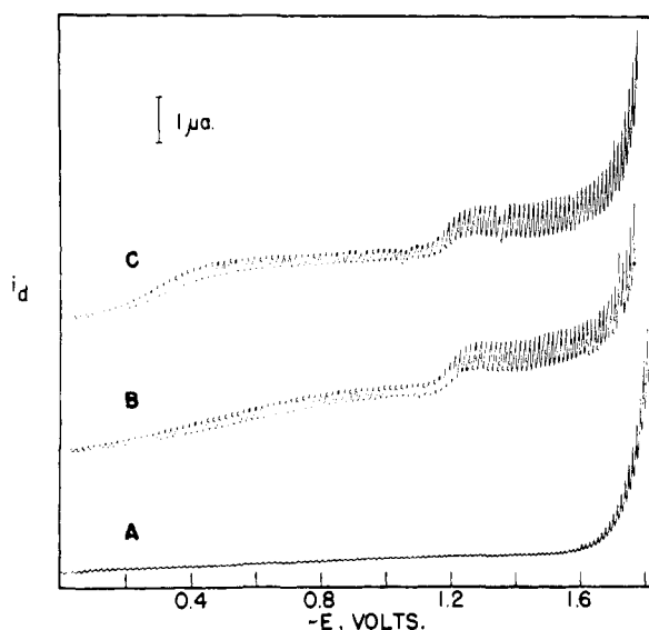
Fig. 3.—Polarograms for (A) background solution (0.48 M sodium acetate adjusted to pH 5.56 with acetic acid), (B) meso -dibromosuccinic acid (0.261 mM ), and (C) rac -dibromosuccinic acid (0.255 mM ).
