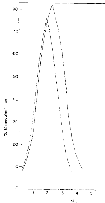
Fig. 5.—Variation of percentage monovalent ion present with pH in solutions of racemic dibromosuccinic acid. The solid line is plotted from calculations made using the ionization constants given by H. Bode and K. Petersen, Ber. , 71B , 871 (1938), assuming unit activity; the broken line represents similar calculations using activities calculated for an ionic strength of 1.0.
